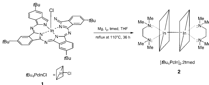
Scheme 1. Synthesis of 2 .
